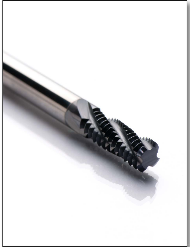
THREAD MILLING
