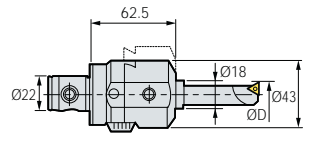
1DIV = Ø0.02 MM
